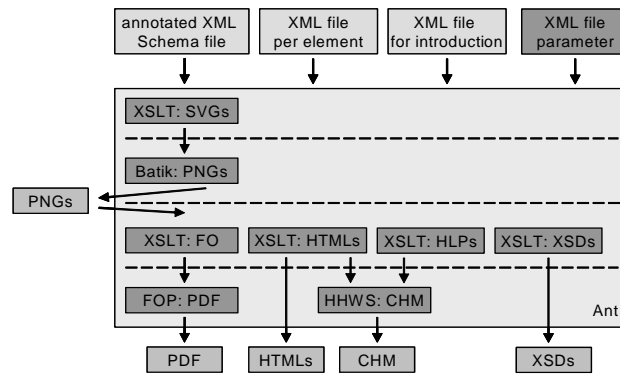
Figure 2. Steps for the automatic creation of the documentation
